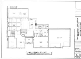
3 Proposed First Floor Plan
